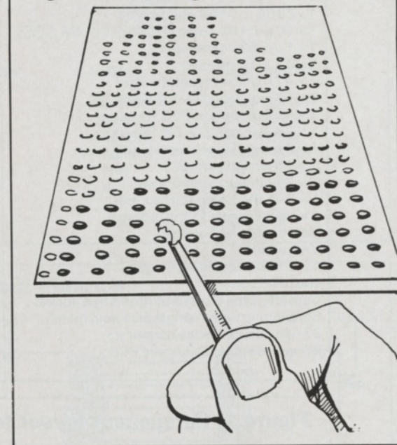
Figure 9: Cutting tracks
